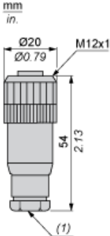
(1) Cable gland : no. 7 plastic (Pg 7)
